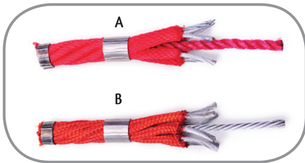
Nylon-core rope (A) vs. steel-core rope (B)
